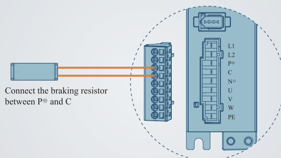
Figure 3-9 Connection of the external braking resistor
