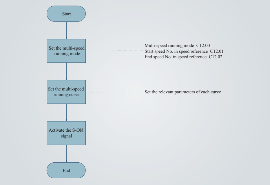
Figure 4-62 Flowchart for setting the multi-speed running function
