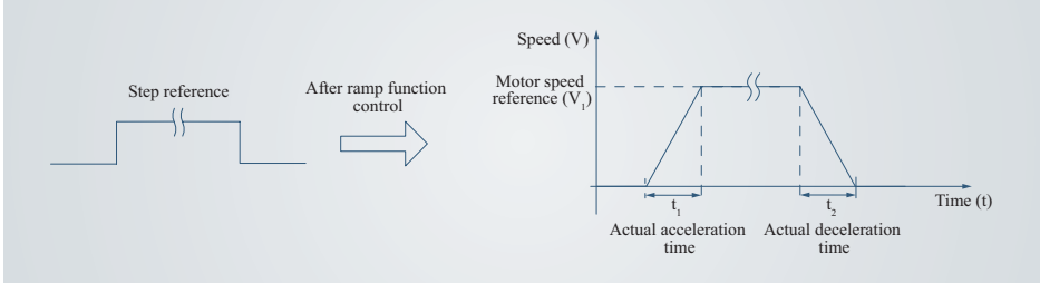
Figure 4-65 Ramp function definition
