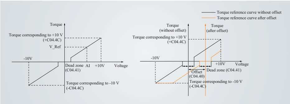
Figure 4-77 AI1 without offset (Left) & AI1 after offset (Right)
