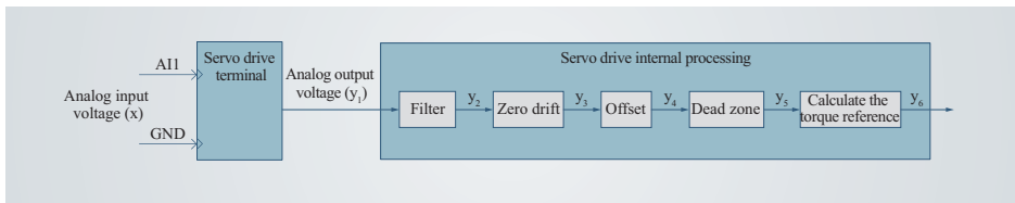
Figure 4-75 AI processing of servo drive
