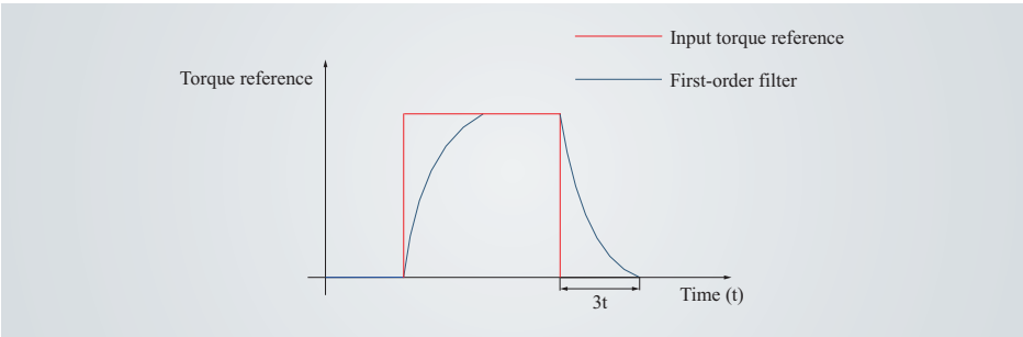
Figure 4-78 First-order filter for rectangular torque references
