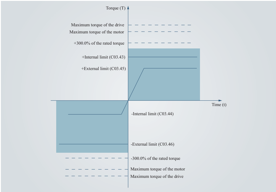
Figure 4-81 Example of torque limit
