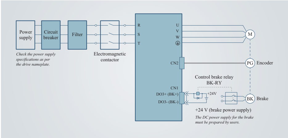
Figure 3-5 Wiring of the brake
