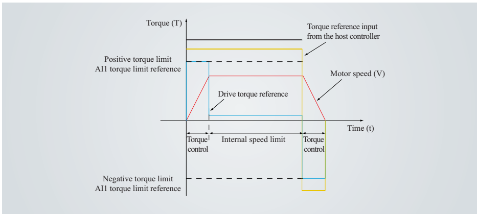
Figure 4-86 AI1 reference torque limit curve
