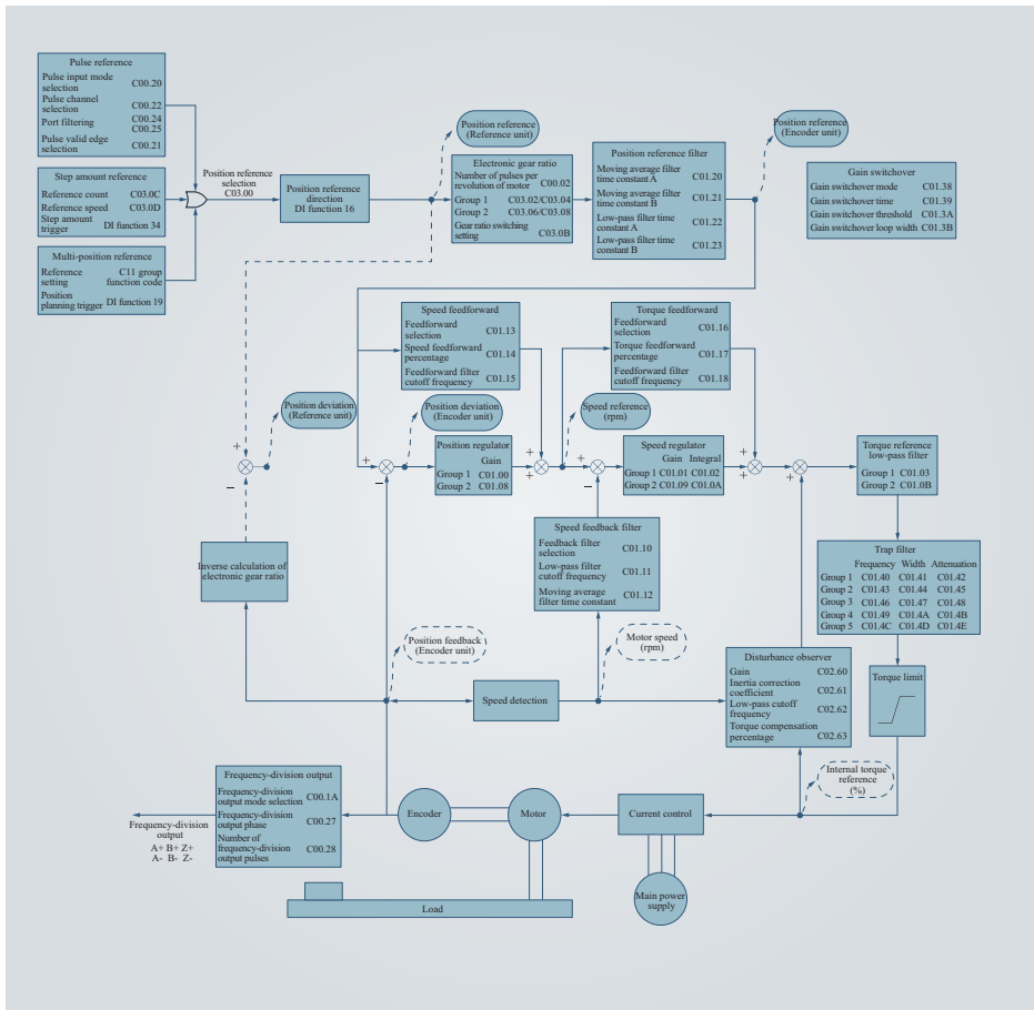
Figure 4-2 Block diagram of function codes in position control mode
