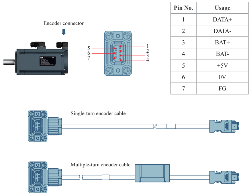
Figure 3-3 Absolute encoder signal cables
