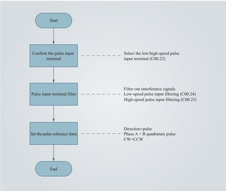
Figure 4-5 Pulse reference source setting flowchart
