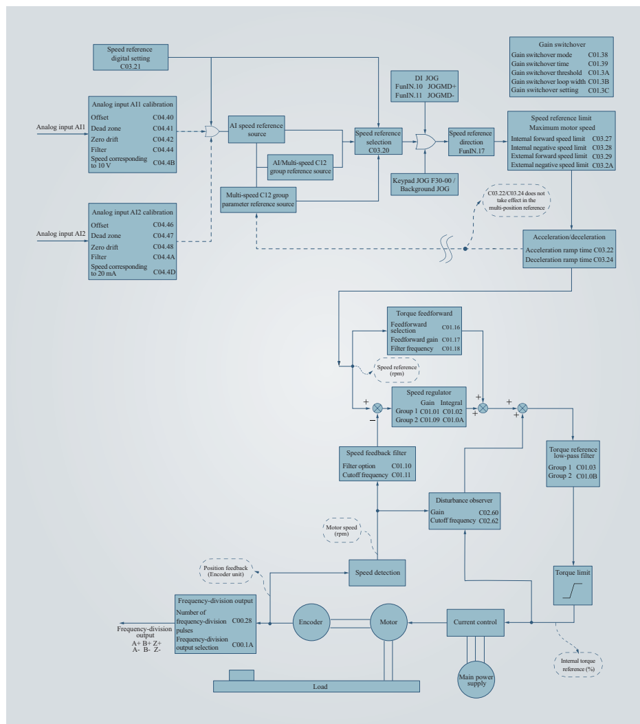
Figure 4-57 Block diagram of speed control mode
