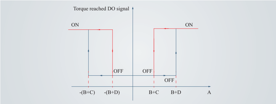
Figure 4-91 Description of torque reached output
