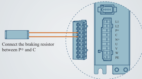
Figure 3-9 Connection of the external braking resistor
