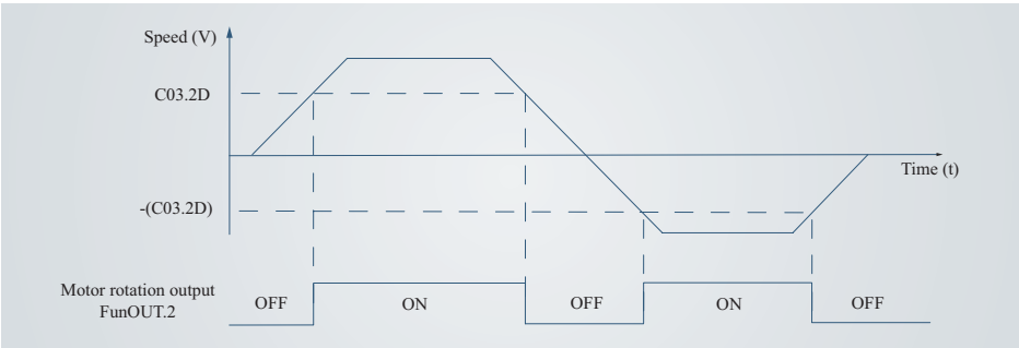
Figure 4-67 Waveform of the motor rotation signal
