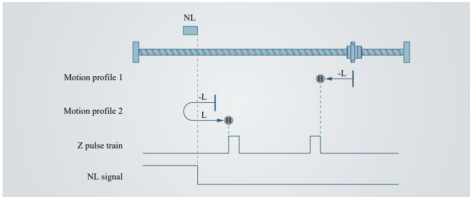
Figure 4-54 Home mode 33 profile and signal status
