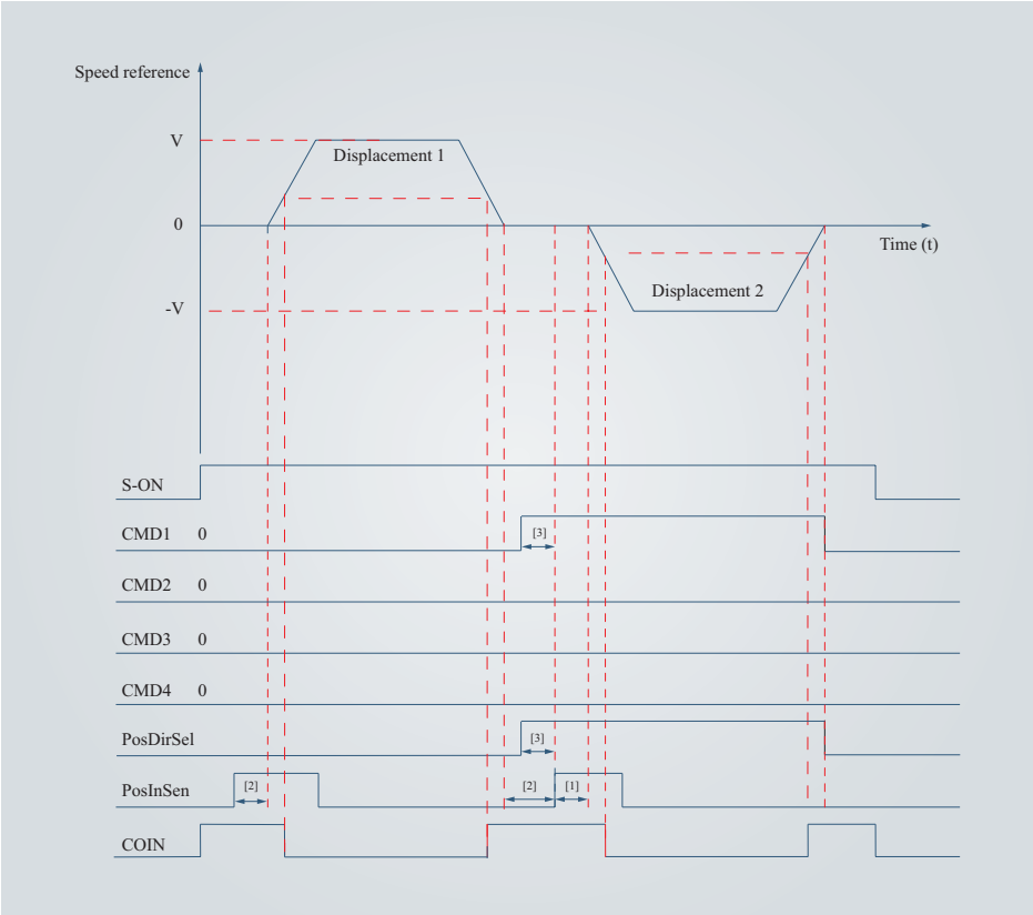
Figure 4-8 Multi-position sequence diagram
