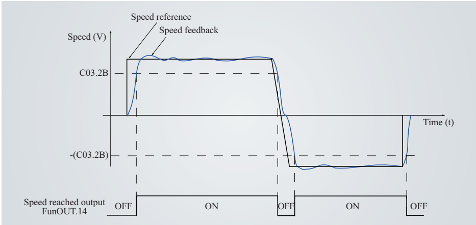
Figure 4-69 Waveform of the speed reached signal
