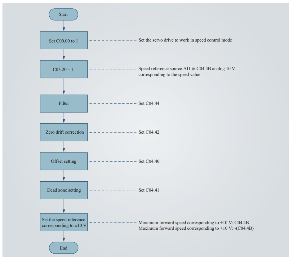
Figure 4-58 Operation flowchart of setting the speed reference by using analog voltage
