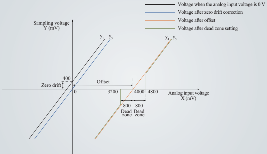
Figure 4-60 Example of sampling voltage for servo drive AI processing
