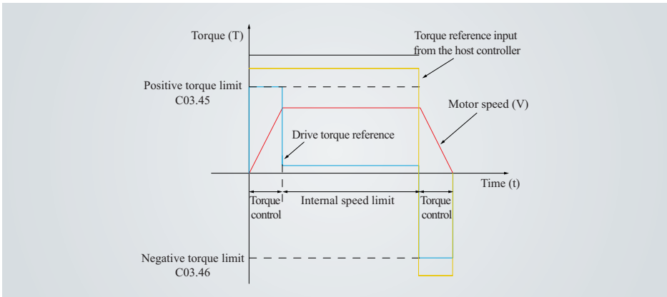
Figure 4-84 Torque limit curve (C03.42 = 1)
