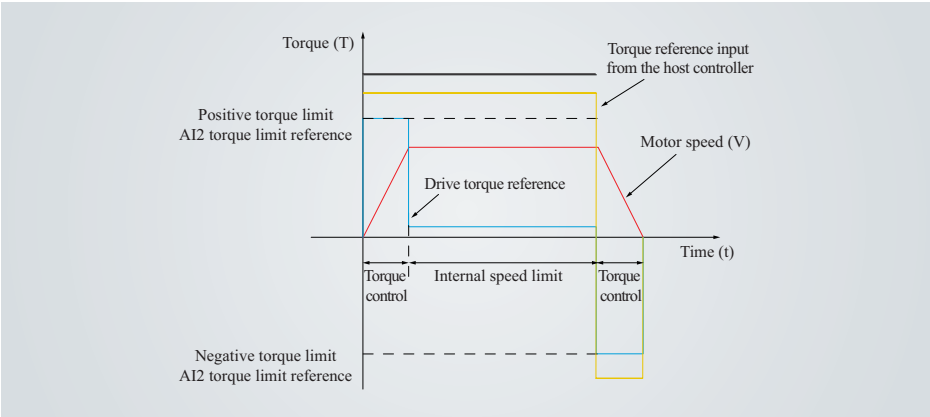
Figure 4-87 AI2 reference torque limit curve
