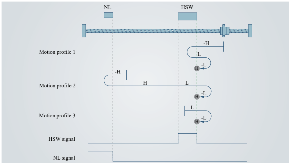
Figure 4-51 Home mode 28 profile and signal status
