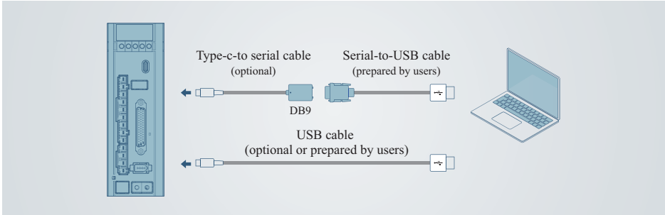
Figure 3-6 Communication terminal connection
