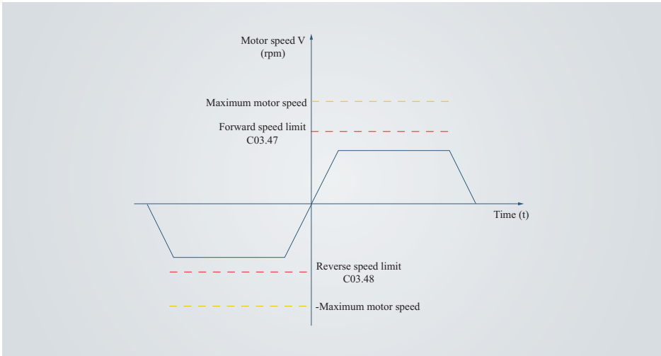
Figure 4-89 Speed limit curve
