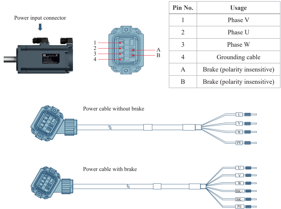
Figure 3-2 Power cable for terminal-type motor
