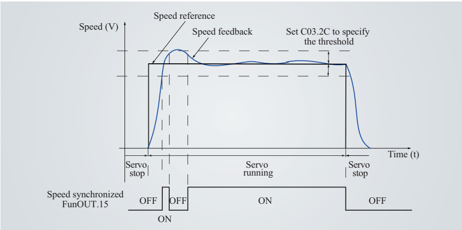
Figure 4-68 Waveform of the speed synchronized DO signal
