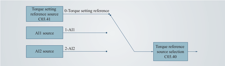
Figure 4-73 Torque reference sources
