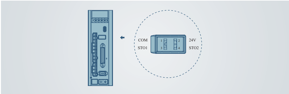
Figure 3-7 Layout of the safety STO terminal
