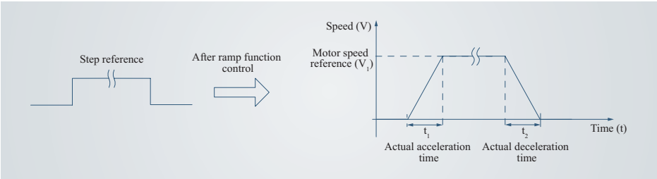
Figure 4-65 Ramp function definition
