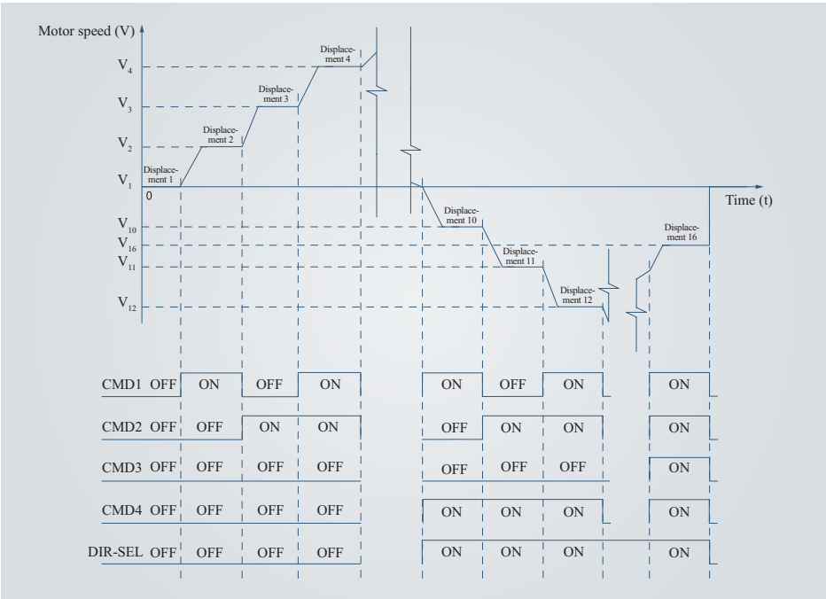
Figure 4-63 Example of multi-speed curve
