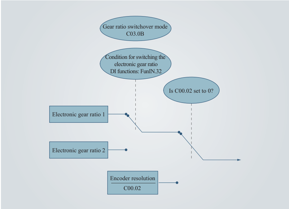
Figure 4-14 Flowchart for setting the electronic gear ratio
