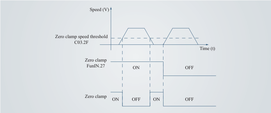
Figure 4-66 Wiring and waveform of zero clamp
