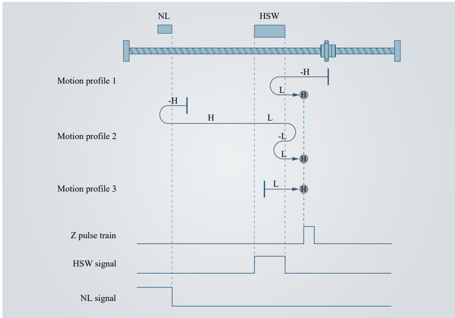
Figure 4-36 Home mode 11 profile and signal status
