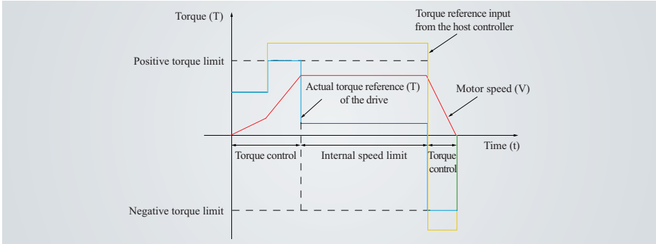
Figure 4-80 Torque setting and torque limit
