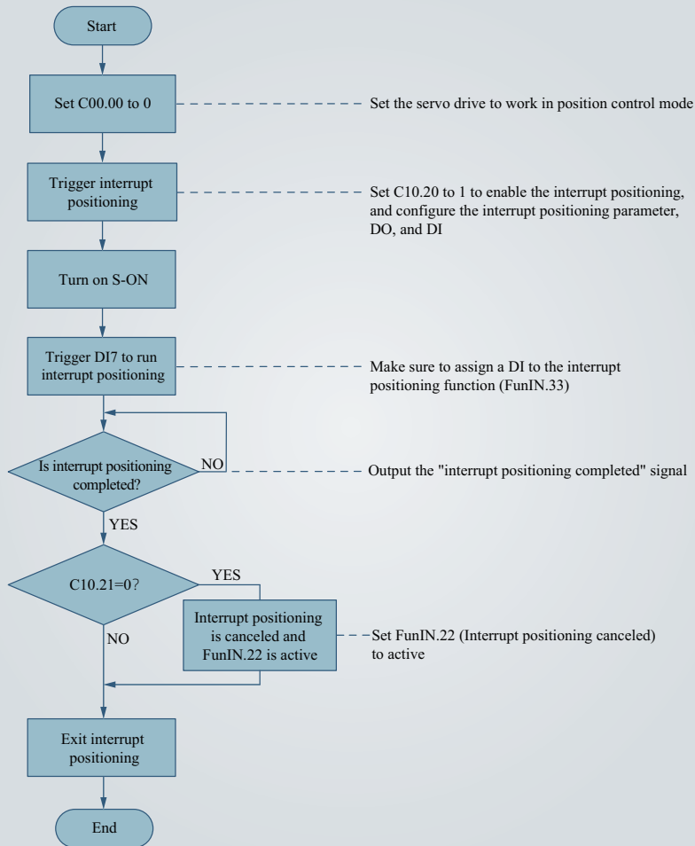
Figure 4-21 Flowchart of the interrupt positioning signal
