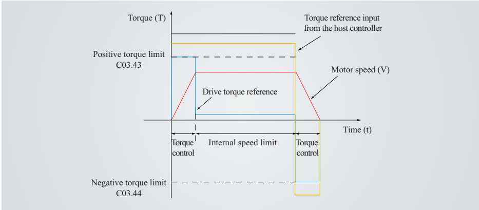
Figure 4-83 Torque limit curve (C03.42 = 0)
