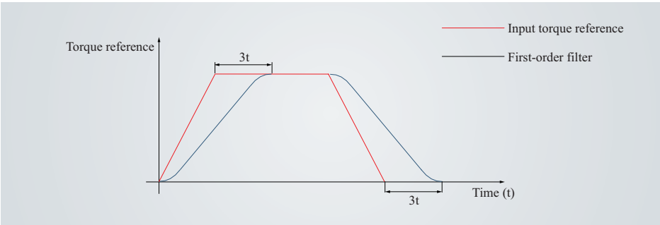
Figure 4-79 First-order filter for trapezoid torque references
