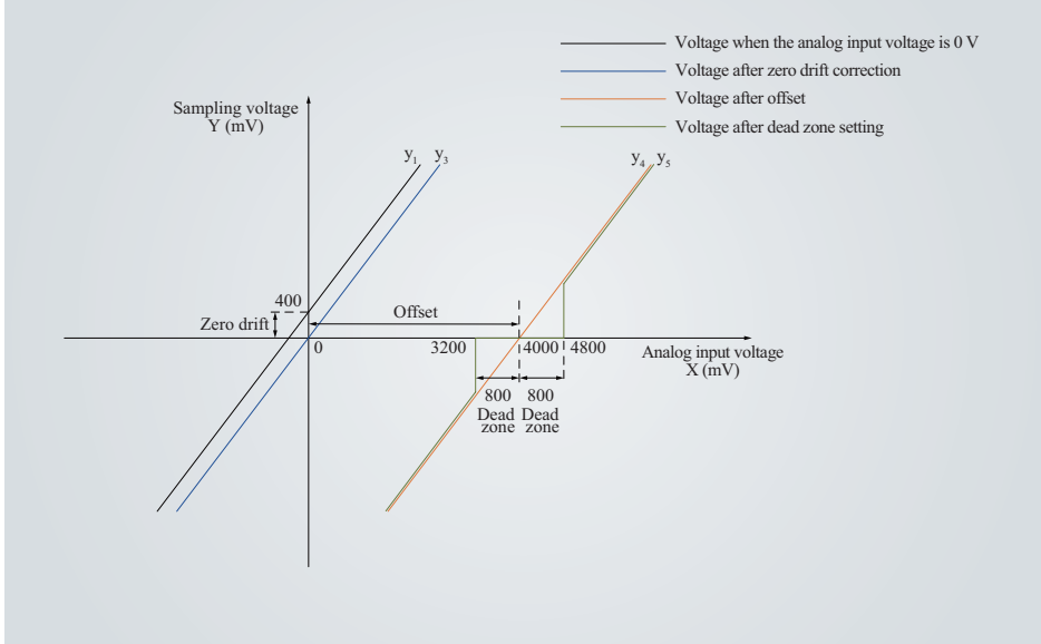
Figure 4-76 Example of sampling voltage for servo drive AI processing
