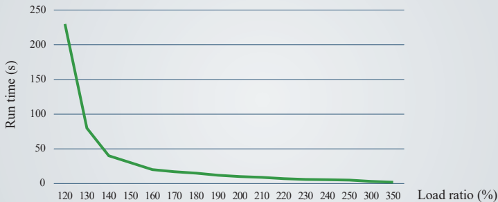
Figure 10-4 Motor overload protection curve
