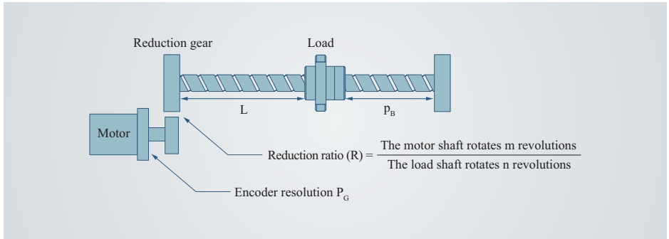
Figure 4-16 Ball screw
