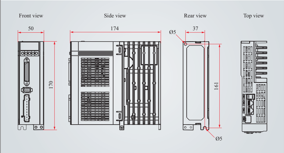
Figure 2-2 Installation dimensions for SIZE B (unit: mm)
