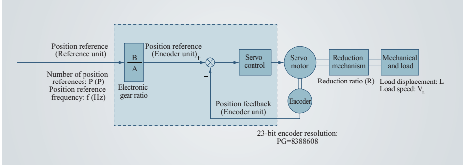
Figure 4-15 Relationship among the position reference (reference unit), load displacement, and electronic gear ratio
