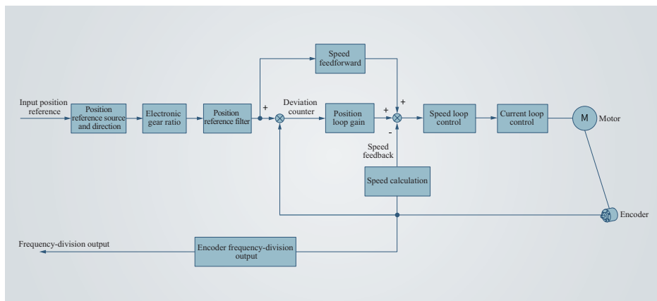
Figure 4-1 Position control block diagram
