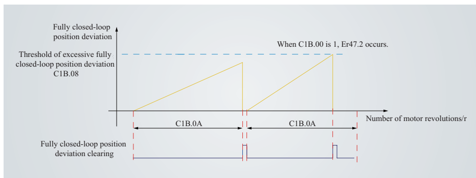
Figure 4-92 Fully closed-loop position deviation clearing description
